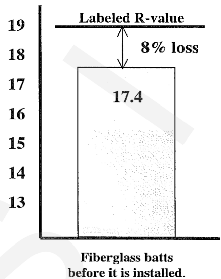
Figure 3 – Before any of the installation tests were begun, the fiberglass batts were tested and found to provide R-17.4
